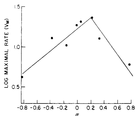
FIGURE 2: Logarithm of the maximal rate ( V_M ) for the substituted phenylalanines as substrates of hog kidney D-amino acid oxidase, plotted against \sigma (see footnote b of Table II). The respective maximal rates, taken from Table III, refer to micromoles of substrate oxidized per minute per milligram of protein at 38° in air.
