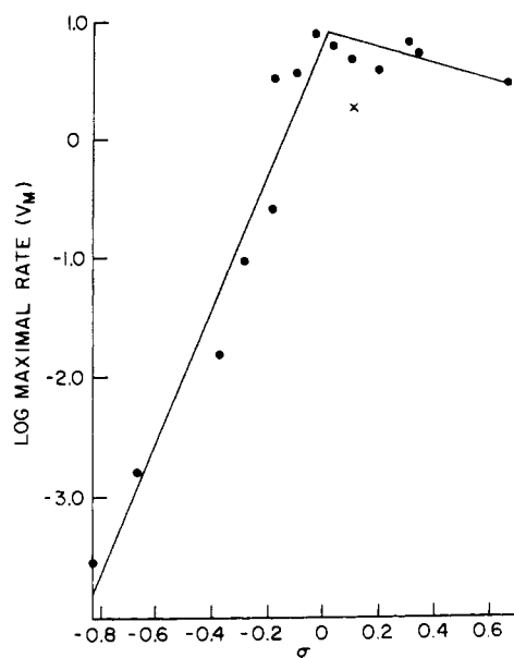
FIGURE 1: Logarithm of the maximal rate ( V_M ) for the substituted C-phenylglycines as substrates of hog kidney D-amino acid oxidase, plotted against \sigma (see footnote b of Table II). The respective maximal rates, taken from Table II, refer to micromoles of substrate oxidized per minute per milligram of protein at 38° in air. x refers to m -methoxy-C-phenylglycine (see text).
