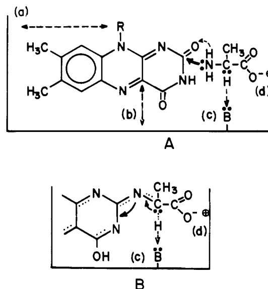
FIGURE 3: Working hypothesis for the interaction between D-alanine and D-amino acid oxidase. One or more linkages between the flavin component and the enzyme-protein are depicted as dashed lines between flavin and (a) and (b). D-Alanine is used as a model substrate. See text for further details. (Figure appeared as Scheme 1 in paper II, Coffey et al. (1965); reproduced by permission.)
